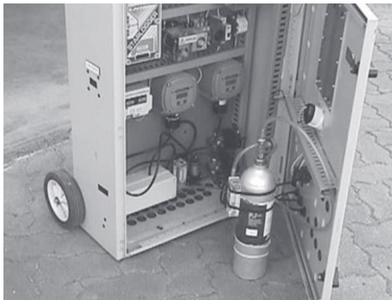
Figure 4: Gas monitoring machine in operation.
