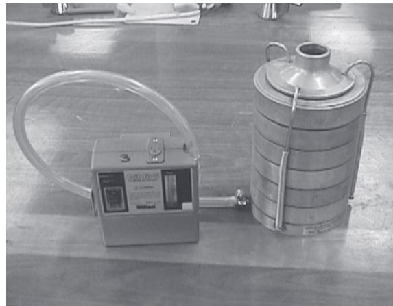
Figure 3: Anderson sampler.
