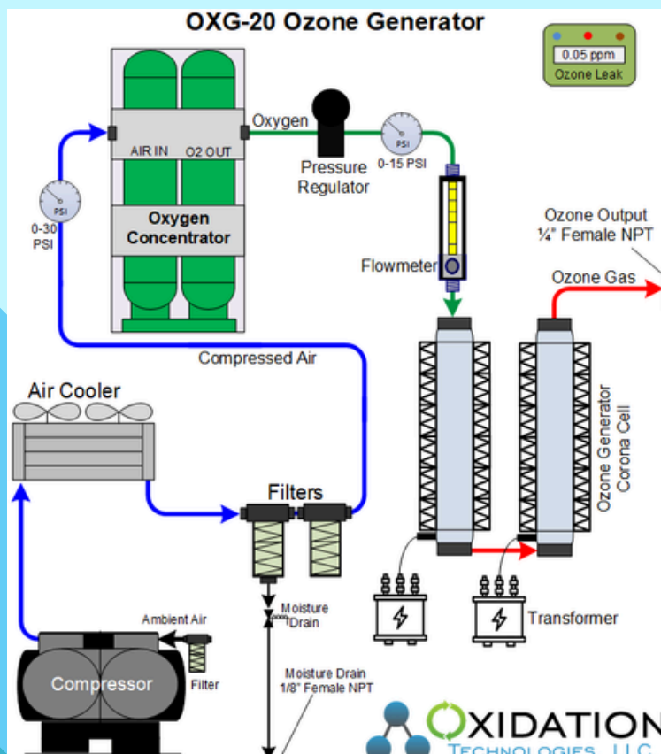
Standard OXG-20 Diagram
