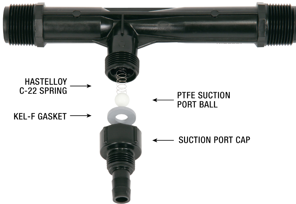
PTFE Suction Port Ball, Kel-F Gasket and Hastelloy C-22 Spring
