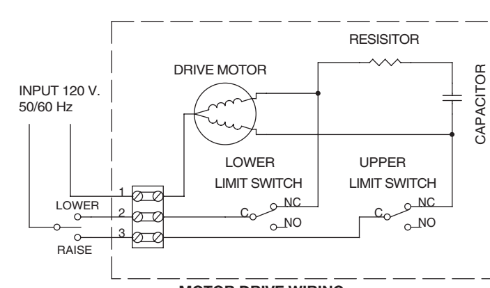
MOTOR DRIVE WIRING FIGURE G
