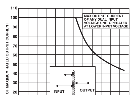
OPERATION IN "STEP-UP" CONNECTION FIGURE F
